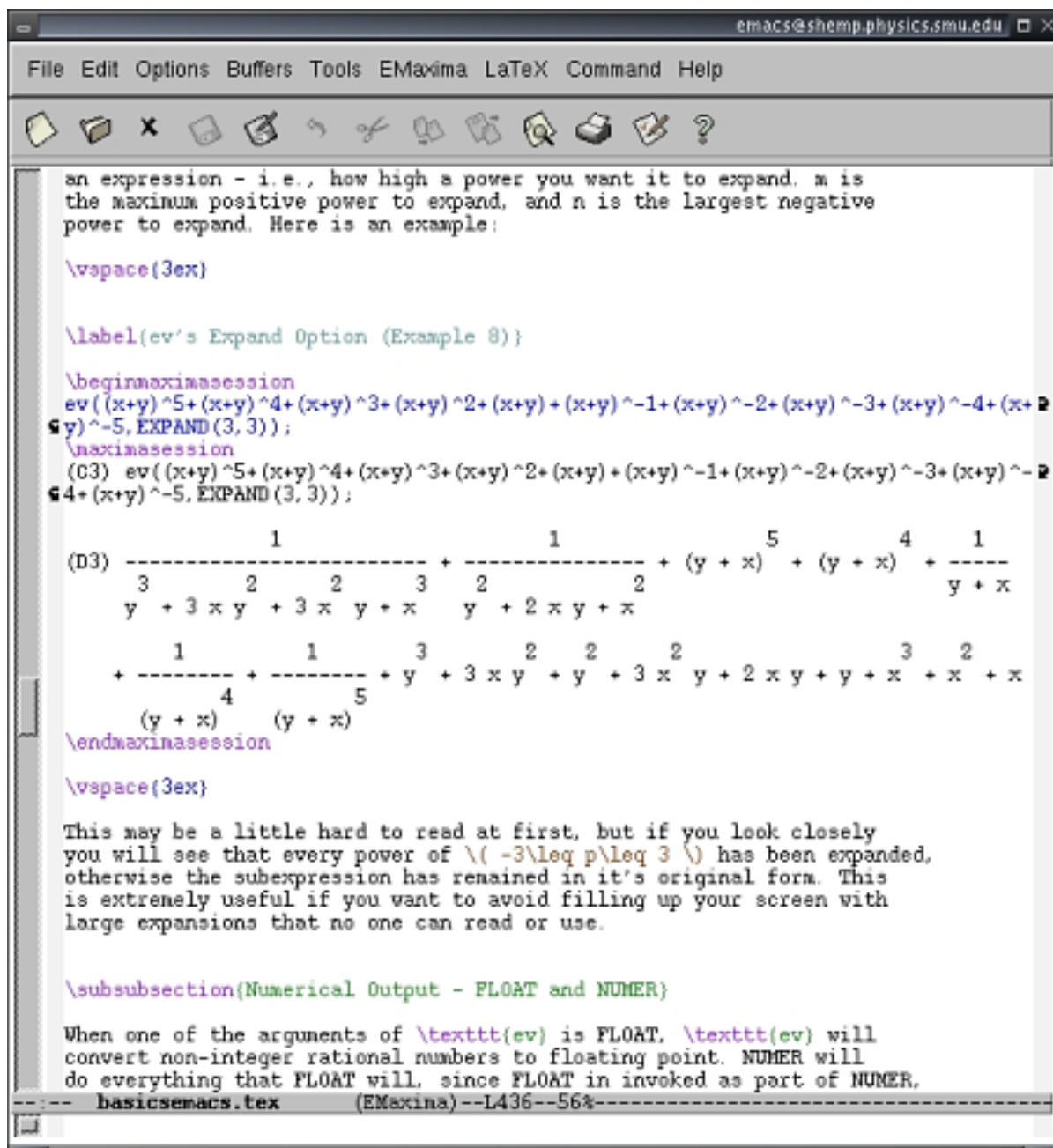
Figure 2.3: An Emaxima Session
